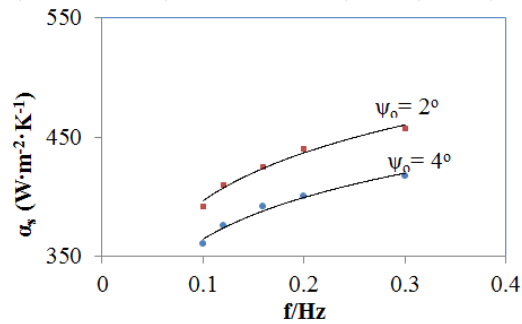
Heat transfer coefficient and vibration frequency under different inclination angles
