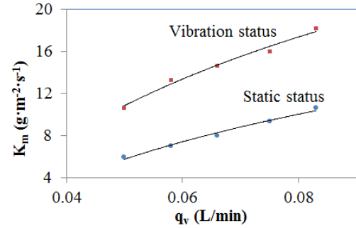
Mass transfer coefficient and solution sprinkling rate
