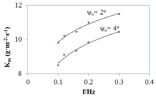
Mass transfer coefficient and vibration frequency under different inclination angles
