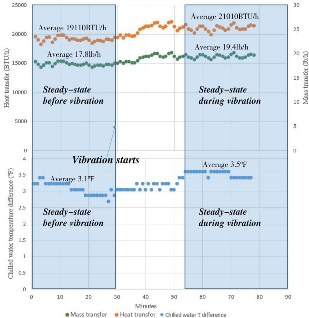
Heat and mass transfer &amp; chilled water temperature difference (IP)
